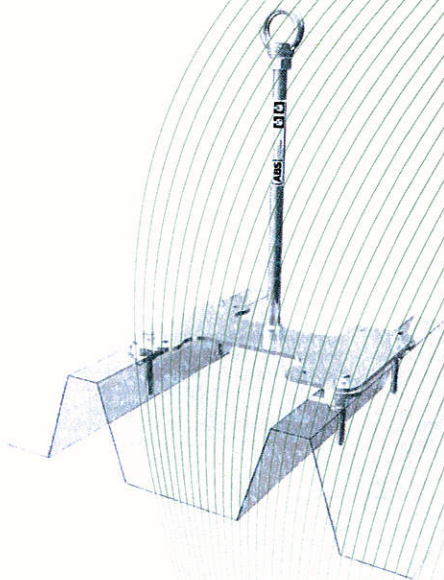
Fig. 1: Anchor device of type ABS-Lock® X-SW
